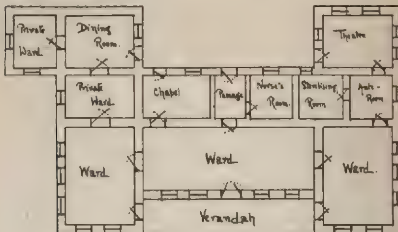
FIG. 326.—Plan of St. Agatha's Hospital, Pingyin, Shantung.
