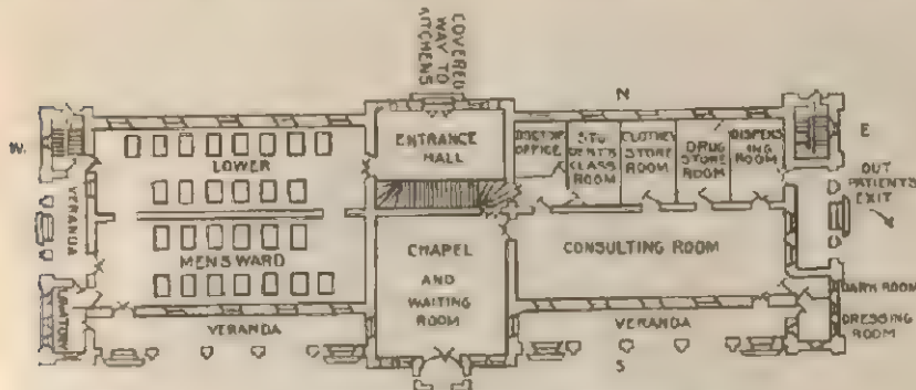
FIG. 231.—Free Methodist Mission Hospital, Wenchow. Ground floor.
