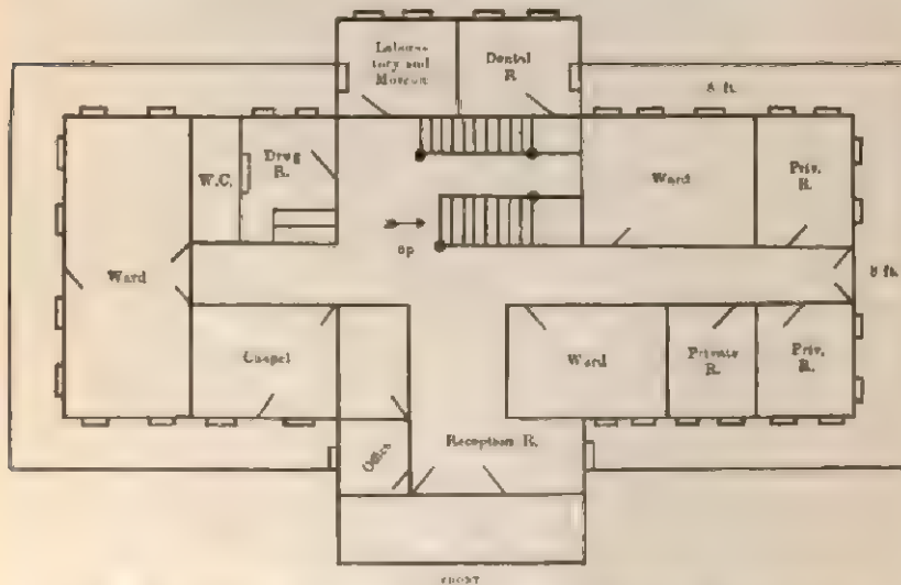
FIG. 344.—Plan of the Methodist Episcopal Hospital for Men, Chungking.
