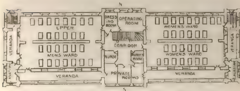
FIG. 232.—Free Methodist Mission Hospital, Wenchow. First floor.
