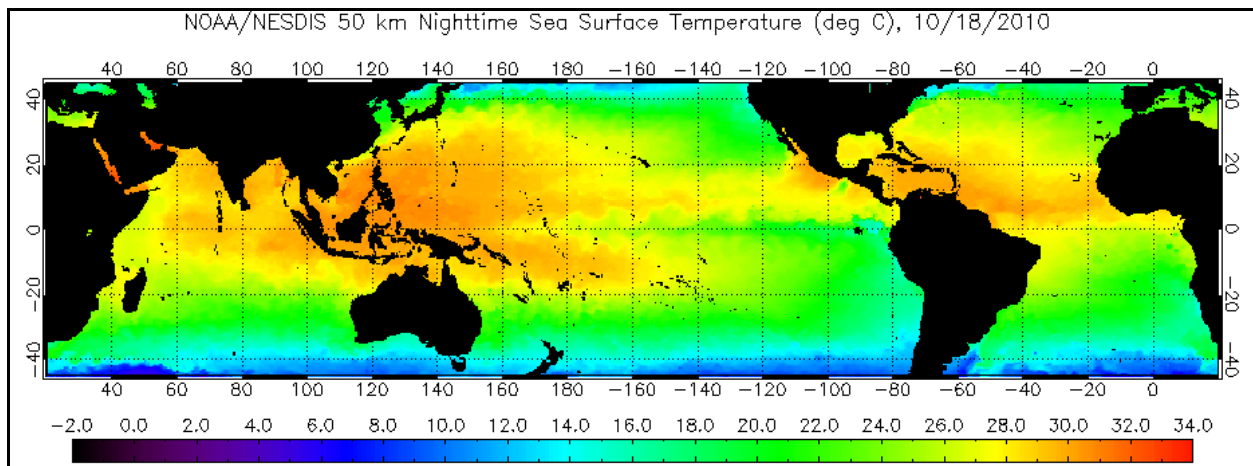
Figure 1. CRW's operational near-real-time twice-weekly global 50 km nighttime SST analysis for October 18, 2010.
