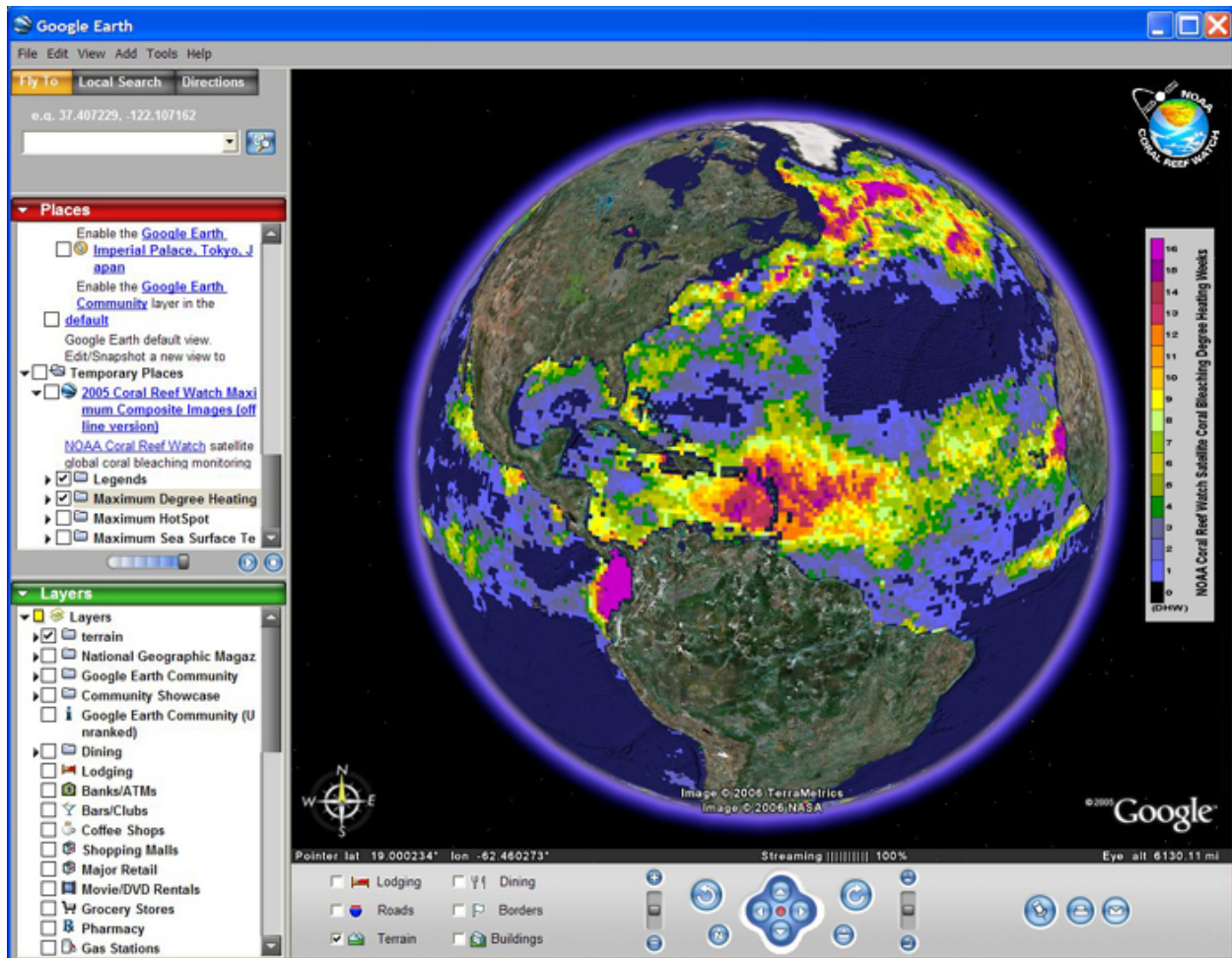
Figure 14. Google Earth display of the maximum composite of CRW's 50 km satellite Coral Bleaching Degree Heating Weeks (DHW) during the 2005 record-breaking mass coral bleaching event in the Caribbean.
