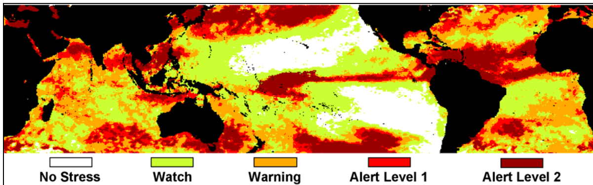
Figure 7. Annual maximum composite of NOAA Coral Reef Watch's operational twice-weekly 50 km satellite Bleaching Alert Areas product for 2010, indicating areas where bleaching thermal stress levels were observed (Table 1).
