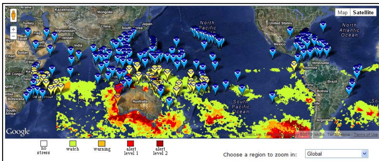
Figure 9. Google Map display of CRW's 24 operational and 227 experimental Virtual Stations for March 4, 2013 with the Bleaching Alert Area image of the same date in the background.
