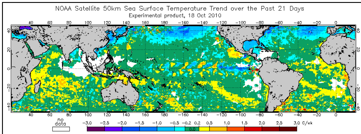
Figure 6. CRW's experimental near-real-time twice-weekly global 50 km Short-Term SST Trends product for October 18, 2010.
