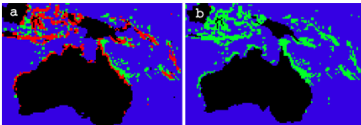
Figure 17. Comparison of CRW's (a) operational 50 km land mask and (b) enhanced 50 km (E-50) land mask for Australia and surrounding regions. Black pixels: land pixels (no data provided); Blue pixels: water pixels (i.e., data pixels); Red pixels: pixels masked as land containing coral reefs (no data provided); Green pixels: water pixels containing coral reefs.
