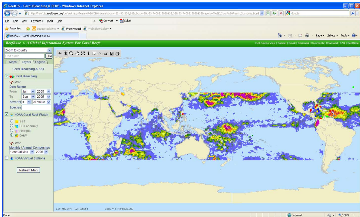
Figure 15. ReefGIS display of the 2005 annual maximum composite of CRW’s twice-weekly 50 km satellite coral bleaching Degree Heating Weeks (DHW).
