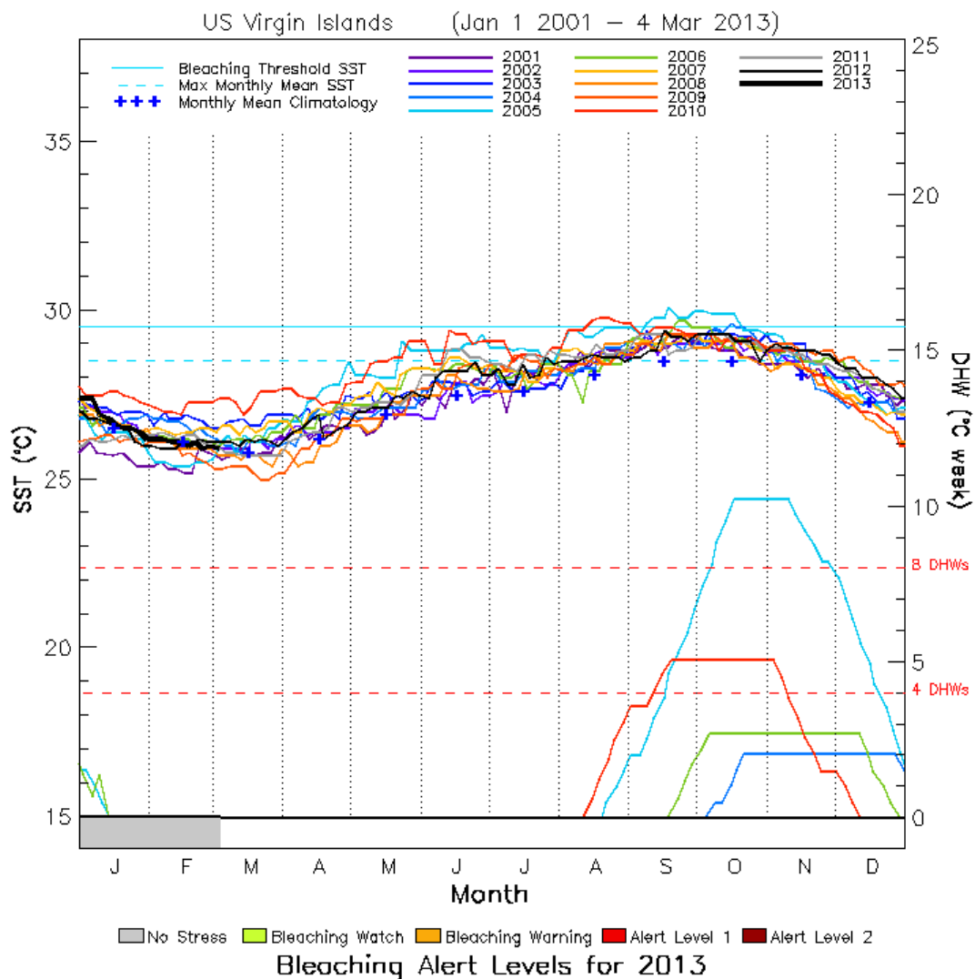
Figure 11. CRW's 2001-2013 multi-year time series graph for the Virtual Station at U.S. Virgin Islands (satellite pixel location between St. Croix and St. John).
