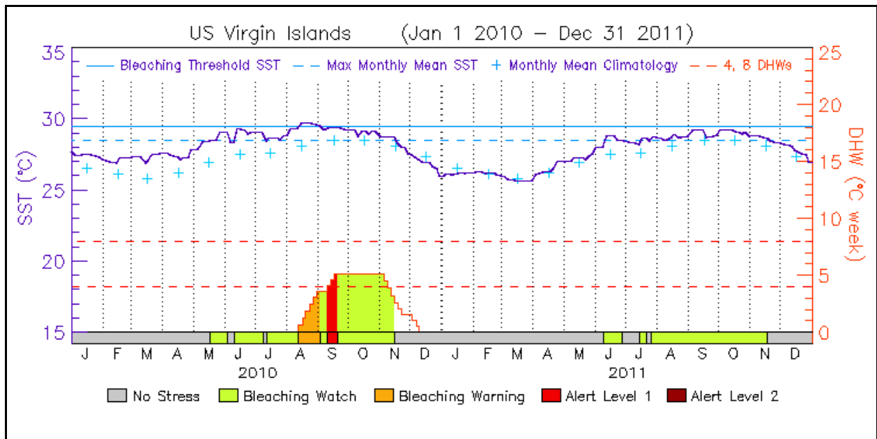
Figure 10. CRW’s 2010-2011 two-year time series graph for the Virtual Station at U.S. Virgin Islands (satellite pixel location between St. Croix and St. John).
