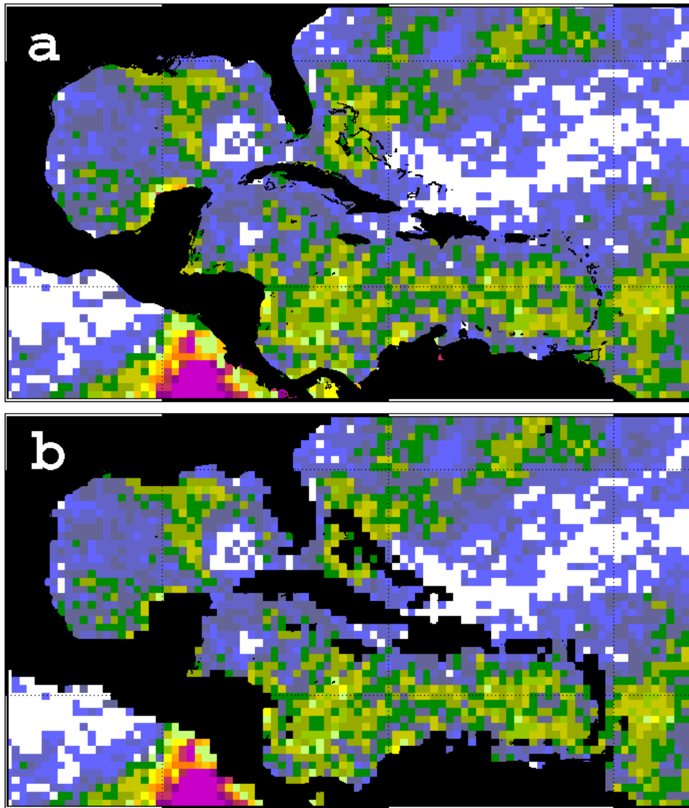
Figure 18. Comparison of CRW's (a) enhanced 50 km (E-50) land mask and (b) operational 50 km land mask for the Caribbean on a sample composite Degree Heating Weeks image.
