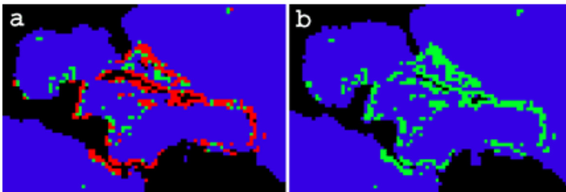
Figure 16. Comparison of CRW's (a) operational 50 km land mask and (b) enhanced 50 km (E-50) land mask for the Caribbean and surrounding regions. Black pixels: land pixels (no data provided); Blue pixels: water pixels (i.e., data pixels); Red pixels: pixels masked as land containing coral reefs (no data provided); Green pixels: water pixels containing coral reefs.
