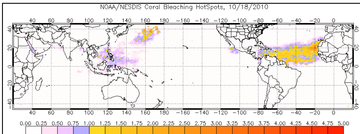
Figure 3. CRW's operational near-real-time twice-weekly global 50 km Coral Bleaching HotSpots for October 18, 2010.
