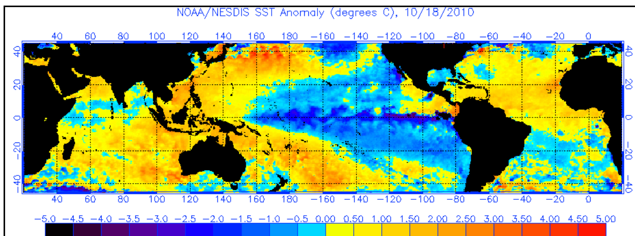
Figure 2. CRW's operational near-real-time twice-weekly global 50 km nighttime SST Anomaly for October 18, 2010.
