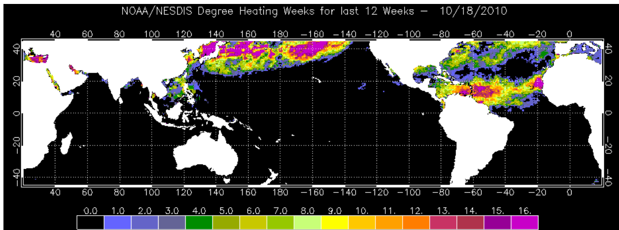
Figure 4. CRW's operational near-real-time twice-weekly global 50 km Coral Bleaching Degree Heating Weeks for October 18, 2010.
