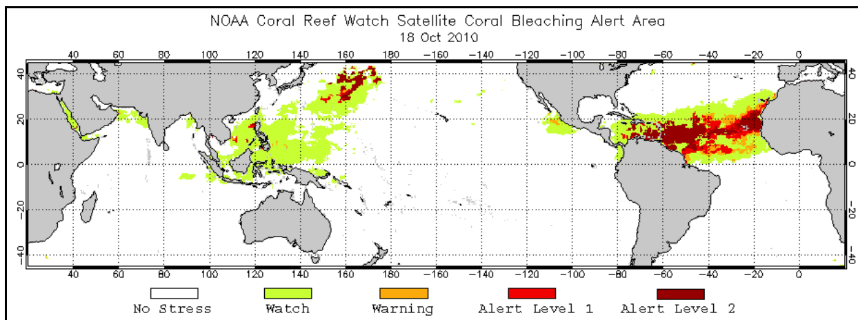
Figure 5. CRW's operational near-real-time twice-weekly global 50 km Bleaching Alert Area for October 18, 2010.
