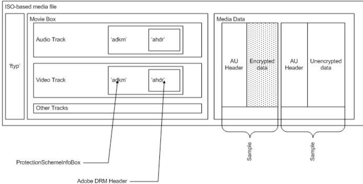
Figure 1 – Example on storing the protection information in F4V
