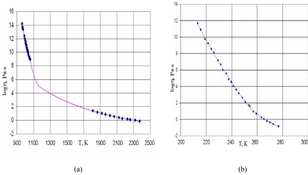
Figure 1. Viscosity-temperature relationships for (a) diopside and (b) salol.
