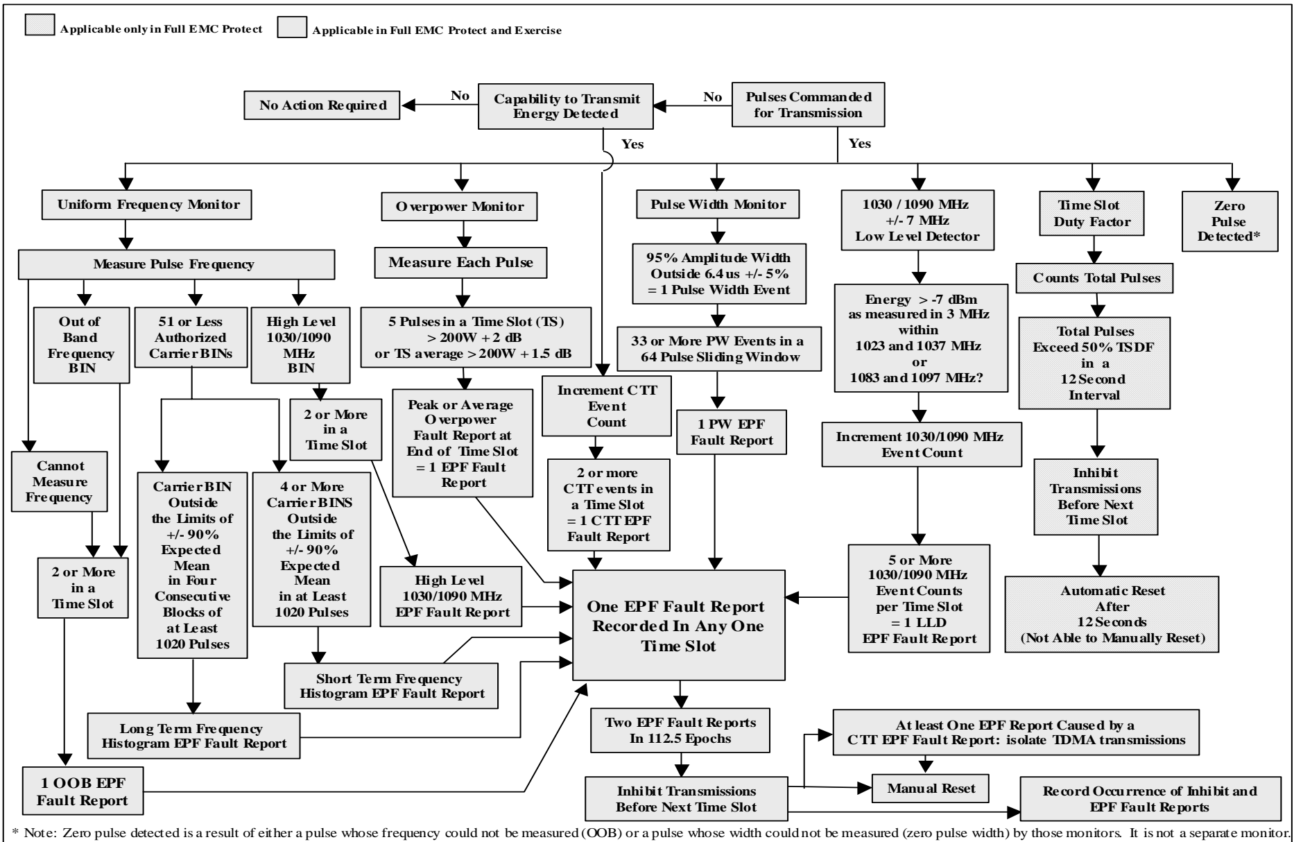
Figure AP1.F3. TDMA Terminal EMC Features Transmit Inhibit Criteria.
