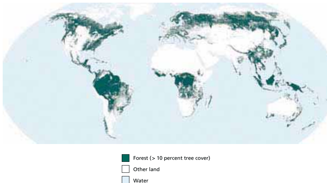
FIGURE 2.1 The world's forests
