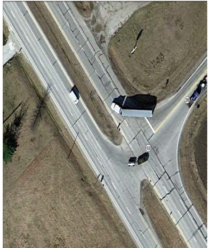
Typical legs of the offset T intersection at US52 and SR28, shown above.
