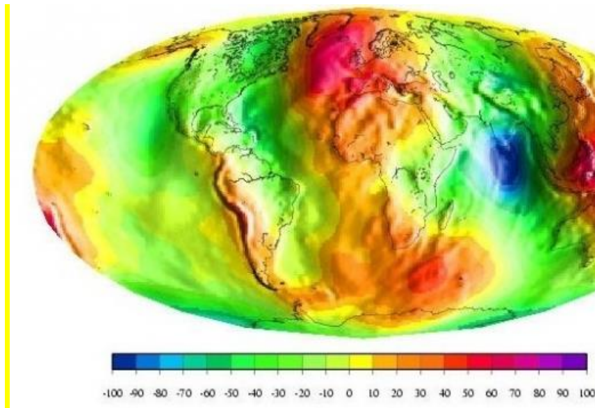
Figure 13 : EGM2008 geoid
