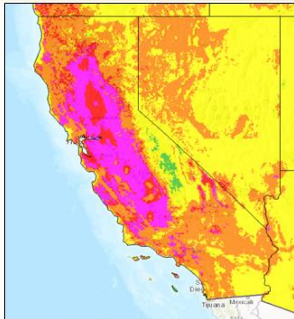
Algorithm Combines MaxT & MinT Values into Final HeatRisk Product
