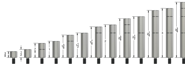
Figure 10 - Possible Standoff Height Increments
