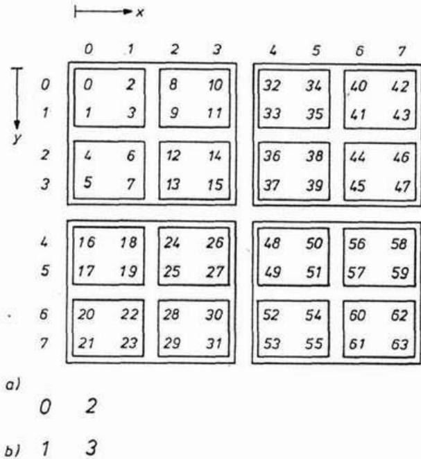
Fig. 6 Bitwise interlacing is a recursive coding scheme
