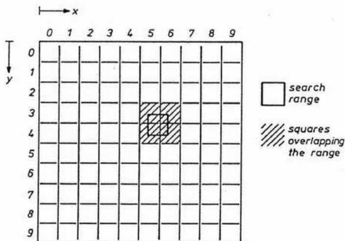
Fig. 3 Dividing the plane into coarse squares. Here, only the squares overlapping the search range must be inspected
