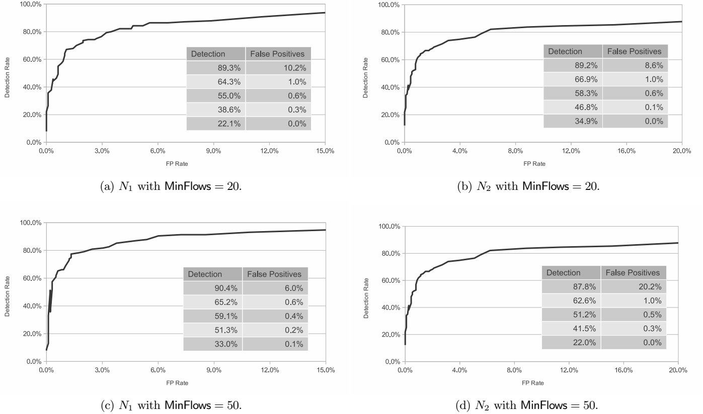
Figure 4: Classification accuracy for each data set ( N_1 and N_2 ) with \text{MinFlows} \in \{20, 50\} .
