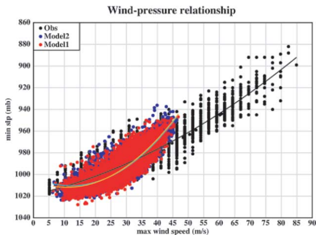
FIG. 4. Scatterplot of maximum surface wind speed ( m s -1 ) versus minimum central surface pressure (h Pa) for observed (black) and simulated (red = Model1; blue = Model2) Atlantic TCs (1980–2006). Model1 data are for 1980–2005. Solid lines are least squares quadratic best-fit lines to the points.
