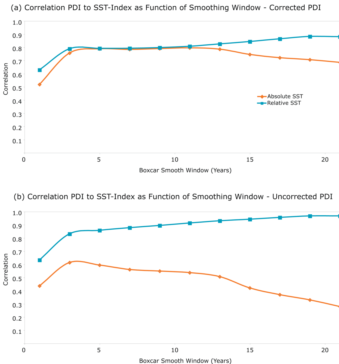
Supplement Figure 2: The top panel is the correlation between the absolute and relative SST time series and the hurricane activity PDI time series based upon HURDAT intensity data corrected as in Supplement Reference 3. The abscissa marks the averaging time applied to each time series before the correlation is taken. The bottom panel is the same, but for hurricane intensities from HURDAT without the intensity correction of Supplement Reference 3.
