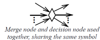
Figure 15.34 Combined MergeNode/DecisionNode notation
