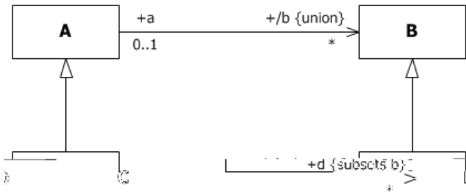
Figure 11.32 Derived supersets (union)
