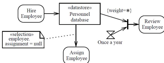
Figure 15.59 DataStoreNode example
