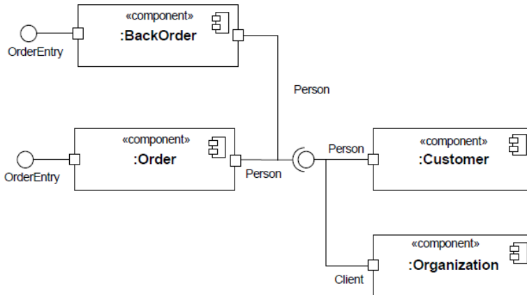
Figure 11.9 An n-ary Connector that assembles four simple Ports using channeled ball-and-socket notation.
