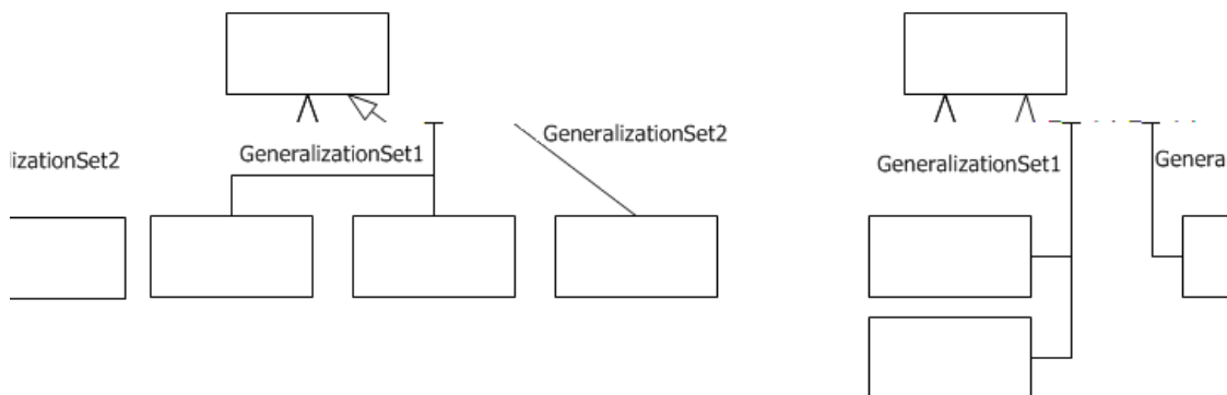
Figure 9.16 GeneralizationSets designated by shared target
