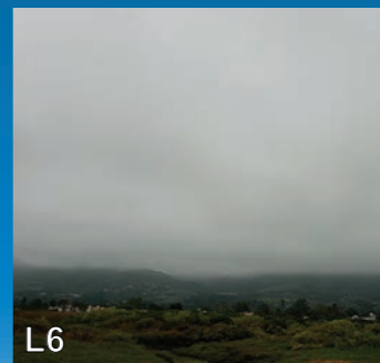
Stratus: In a continuous layer, or Stratus fractus: In ragged shreds, or both, without precipitation.
