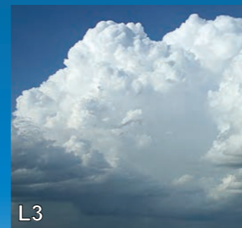
Cumulonimbus: Very tall summits, which lack sharp outlines and are not anvil-shaped.
