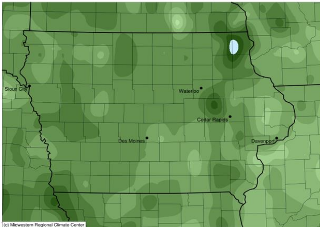
(c) Midwestern Regional Climate Center -10 -9 -8 -7 -6 -5 -4 -3 -2 -1 0 Stations from the following networks used: WBAN, COOP, FAA, GHCN, ThreadEx, CoCoRaHS, WMO, ICAO, NWSLI, Midwestern Regional Climate Center cli-MATE: MRCC Application Tools Environment Generated at: 4/4/2019 9:43:33 AM CDT
