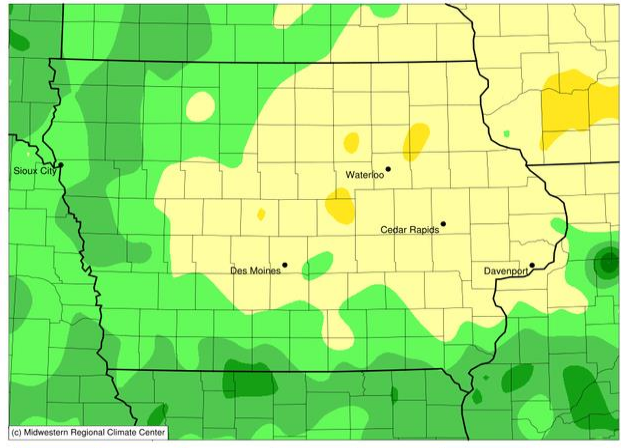
(c) Midwestern Regional Climate Center -1 0 1 2 3 4 Stations from the following networks used: WBAN, COOP, FAA, GHCN, ThreadEx, CoCoRaHS, WMO, ICAO, NWSLI, Midwestern Regional Climate Center cli-MATE: MRCC Application Tools Environment Generated at: 4/4/2019 9:42:23 AM CDT
