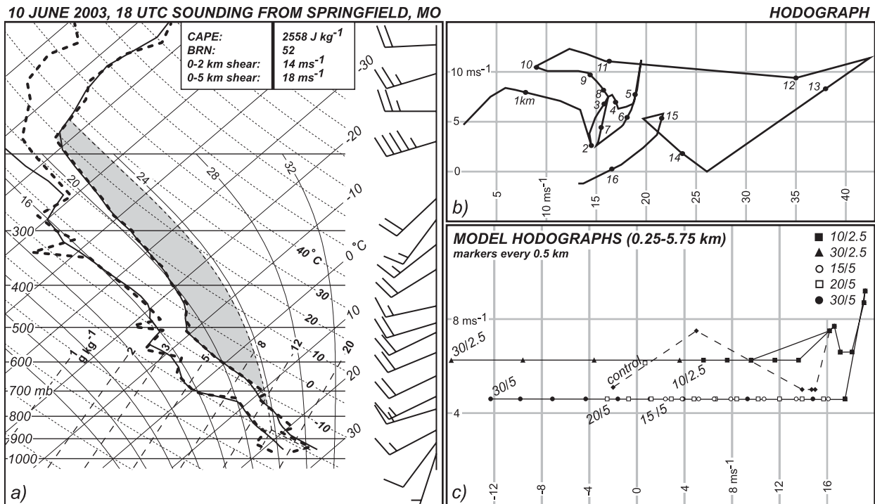
FIG. 2. (a) Skew T -log p and (b) hodograph of the 1800 UTC 10 Jun 2003 Springfield, MO, sounding. The thick dashed lines in (a) are the observed temperature and dewpoint while the thin solid lines are the initial model temperature and dewpoint. The gray shaded area is the CAPE. Winds (half barb = 5 \text{ m s}^{-1} ; full barb = 10 \text{ m s}^{-1} ) are also shown. (c) Hodographs for the low-level and deep shear sensitivity experiments are shown over the lowest 5.75 km.
