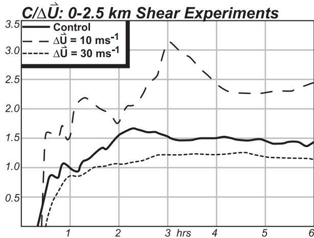
FIG. 7. Time series of C/\Delta U for the low-level (0–2.5 km) shear experiments shown in Fig. 5. Both C and \Delta U are defined in the text.
