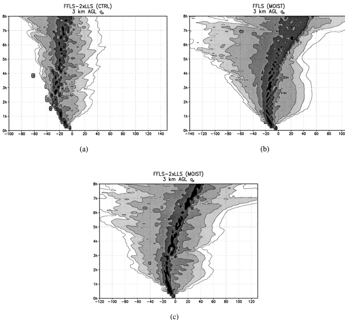
FIG. 18. Same as Fig. 11, but for (a) FFLS-2xLLS simulation with CTRL sounding and (b) FFLS and (c) FFLS-2xLLS simulations with MOIST sounding.
