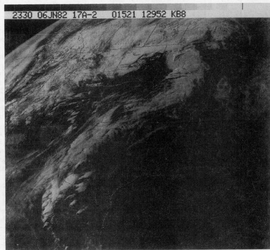
FIG. 1. Enhanced infrared satellite images for (a) 2115 UTC 6 June 1982, (b) (visible image) 2330 UTC 6 June 1982, (c) 0300 UTC 7 June 1982, (d) 0600 UTC 7 June 1982, (e) 0900 UTC 7 June 1982 and (f) 1201 UTC 7 June 1982.
