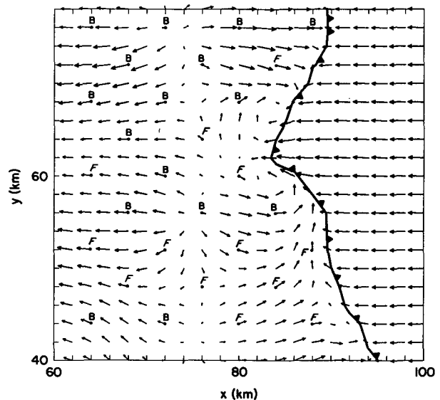
FIG. 16. Map of low-level flow ( z = 350 m) corresponding to Fig. 15. One grid interval represents 16 \text{ m s}^{-1} and the barbed line is the -1 K perturbation potential-temperature contour. The points marked B or F in the cold pool indicate that the air parcels at those points originated either from the back or front side of the line, respectively.
