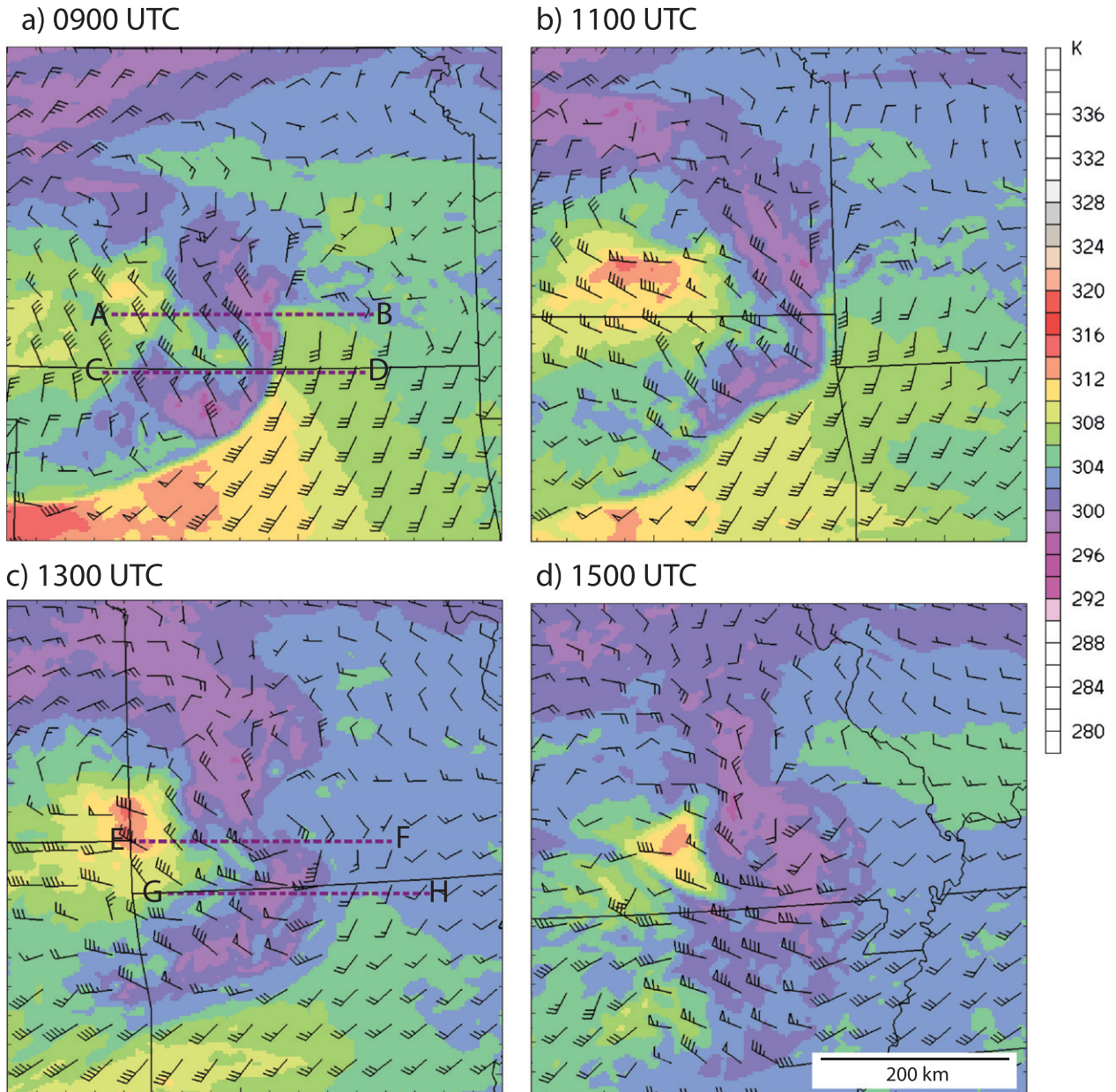
FIG. 10. As in Fig. 9, but at 850 hPa.
