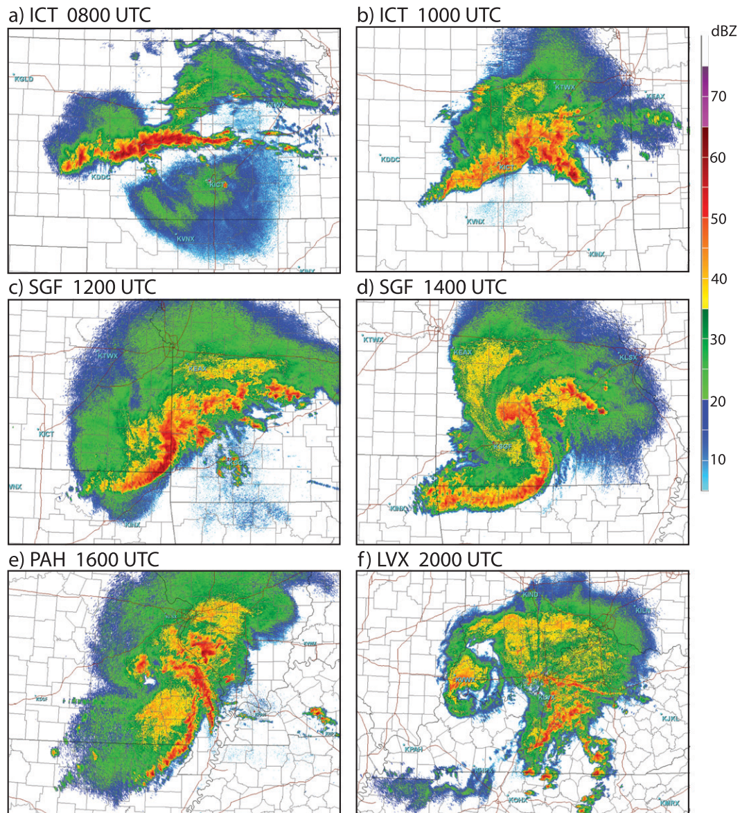
FIG. 2. WSR-88D level II 0.5° radar reflectivity (dBZ; shaded) observed at (a) 0800 and (b) 1000 UTC at Wichita, KS (ICT); (c) 1200 and (d) 1400 UTC at Springfield, MO (SGF); (e) 1600 UTC at PAH; and (f) 2000 UTC at Louisville, KY (LVX), on 8 May 2009.
