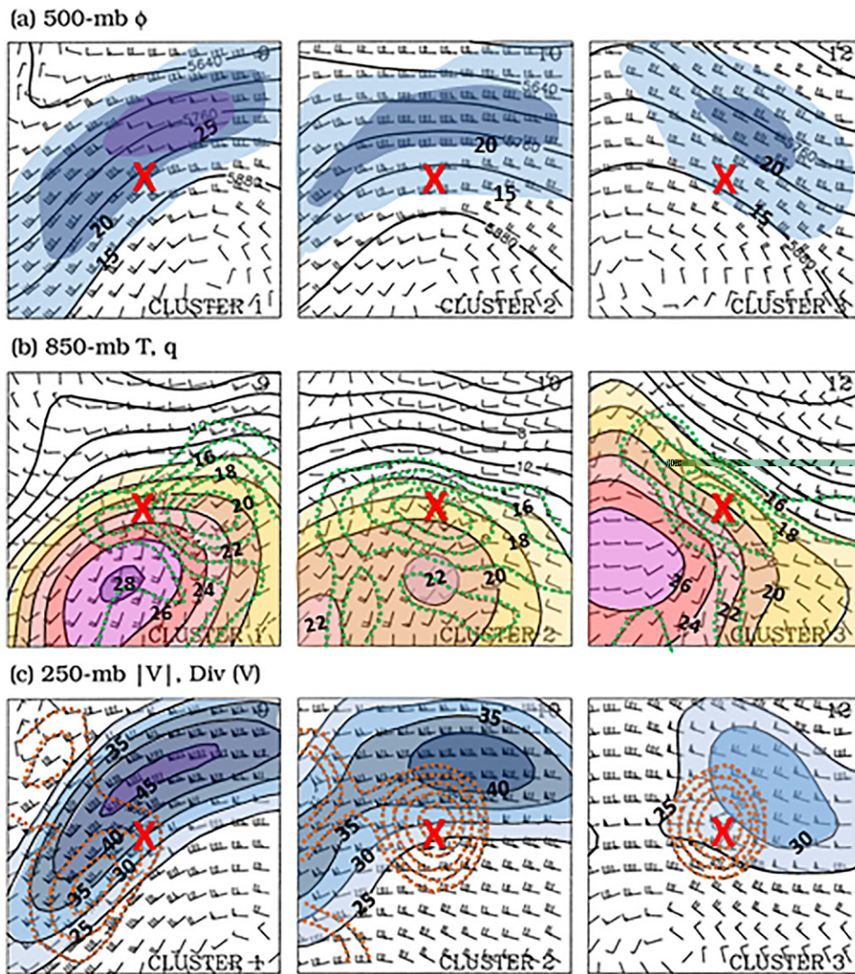
Fig. 14. A composite plot of multiple warm-season DMCS environments driven by upper ridging, showing (a) the mean 500hPa geopotential height ( \phi ; contours every 60m), wind (flag: 50kt or 25 m s -1 ; full barb: 10kt or 5 m s -1 ), and wind speed ( |V| ; shaded every 5 m s -1 , starting at 15 m s -1 ) for three clusters within the upper-ridging pattern. (b) As in (a), but for the 850hPa temperature ( T ; solid contours every 2°C, with shading for values over 16°C) and specific humidity ( q ; green dashed contours every 1 g kg -1 starting at 8 g kg -1 ). (c) As in (a), but for the 250 hPa wind speed ( |V| ; shaded every 5 m s -1 , starting at 25 m s -1 ); divergence of the wind Div(V) ; orange dashed contours every 0.25 \times 10^{-5} s^{-1} ). The horizontal and vertical dimensions of each grid are 2600 km and 2400 km, respectively. The "X" symbol denotes the mean position of the DMCS at the analysis time. The number of cases comprising a cluster for each synoptic pattern (left) 9, (center) 10, and (right) 12. [Subjectively augmented from Coniglio et al. (2004, Fig. 7).]
