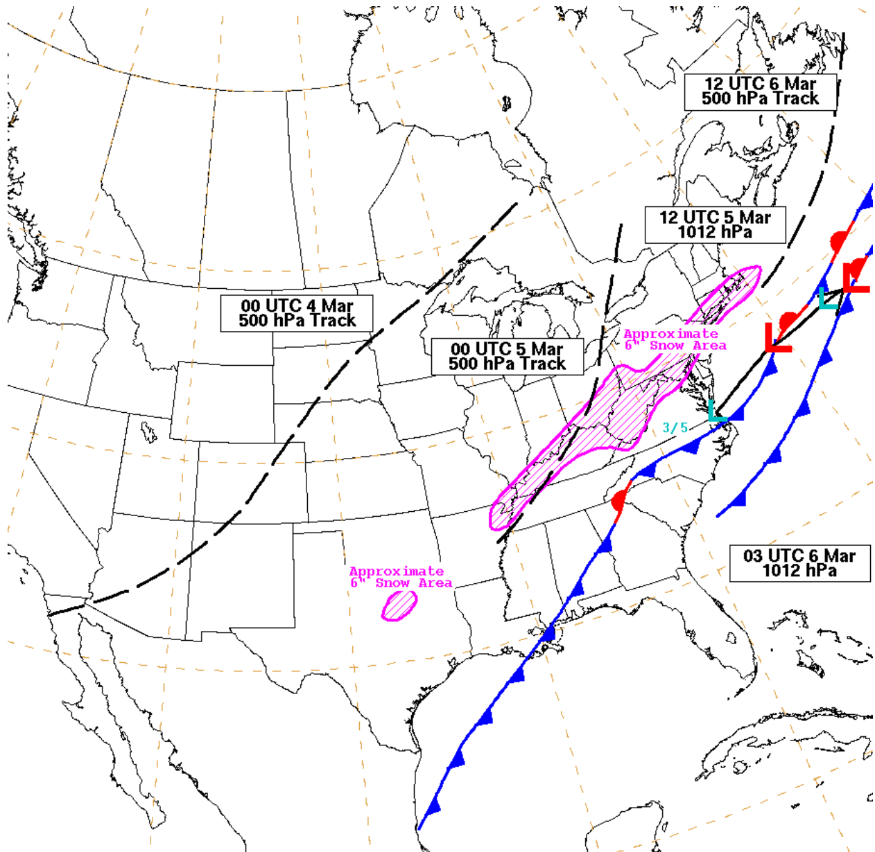
Figure 2: Surface low tracks (cyan), 500 hPa trough (black), and approximate area of greater than 6 inches of snow (pink). The surface frontal analysis at 1200 UTC 05 March and 0300 UTC 06 March is also shown.
