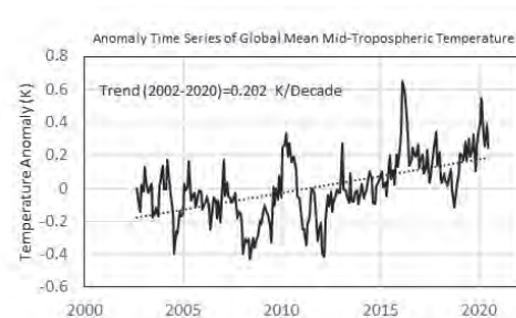
Deseasonalized monthly global mean anomaly time series of mid-tropospheric temperatures merged from Aqua, Metop-A, Suomi NPP, and NOAA-20 satellites. Anomalies are relative to a monthly climatology of the Metop-A period from January 2008 to December 2017. Image credit: C.-Z. Zou, NOAA NESDIS/STAR
