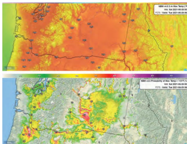
National Blend of Models (top) high temperature forecast and (bottom) probability of high temperature exceeding 110 degrees F for southern Washington and northern Oregon issued 9 pm EDT Friday June 25, 2021, three days ahead of the actual event. Image credit: NOAA NWS Whole Story Uncertainty and Probability (WSUP) Viewer
