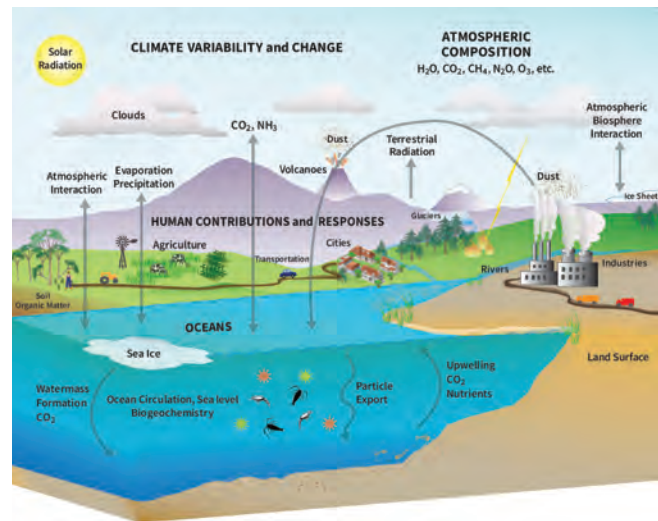
Pictorial representation of the components of and linkages between elements that make up the new Earth System Model. Image citation: Dunne et al. (2020, JAMES, https://doi.org/10.1029/2019MS002015 ) Figure 1
