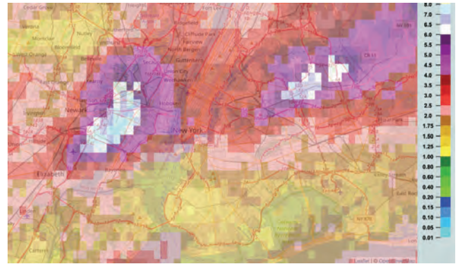
Estimated precipitation in inches from 8 am on June 30 to 8 am on July 3, 2021 over New York City produced by the operational Multi-Radar Multi-Sensor system. Image credit: NOAA Research/NSSL
