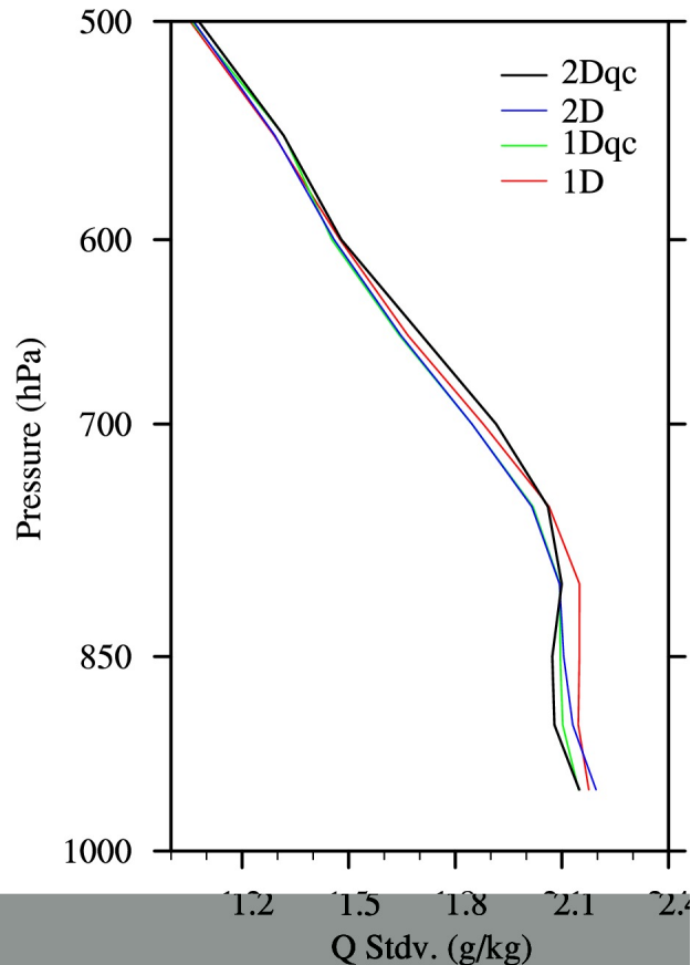
Standard Deviation
