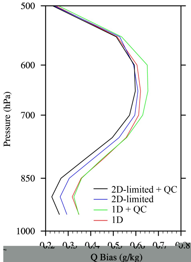
Bias
