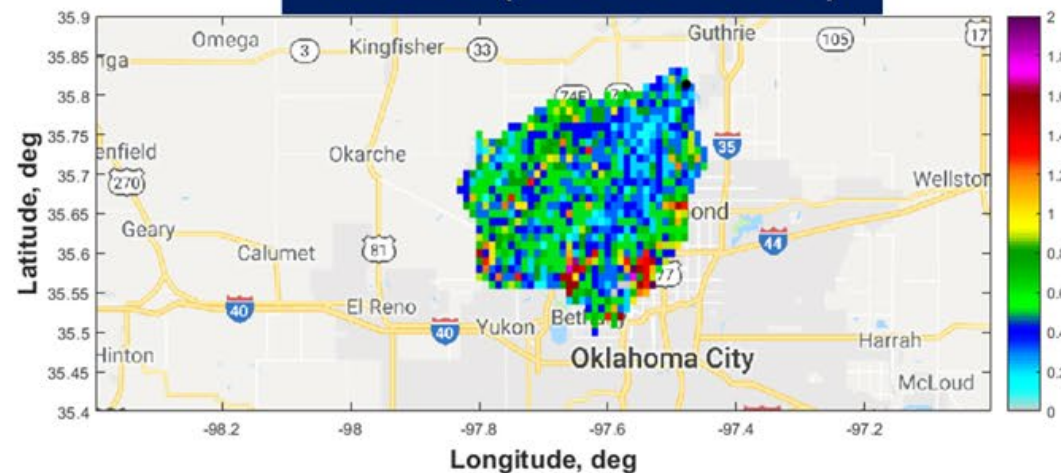
KTLX (5-min/1-km)
