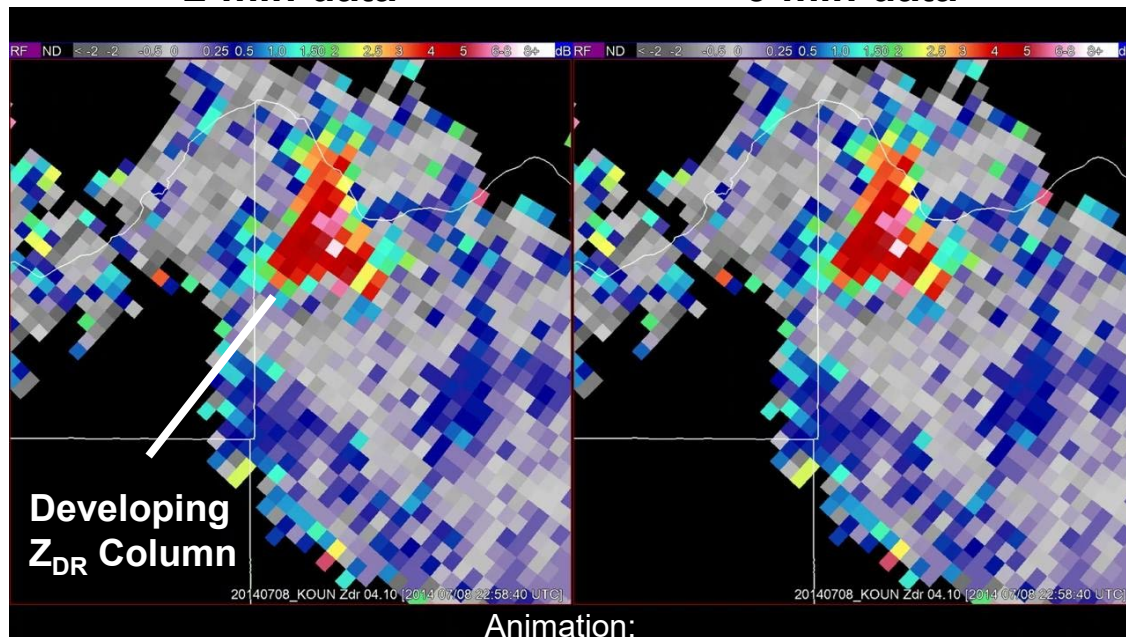
2-min data
