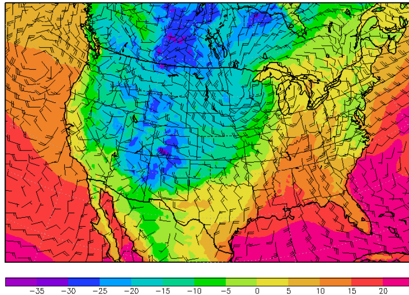
Figure 3: Surface Temperature (°C) and 1000 mb Wind Barbs at 12 UTC on Saturday January 1 st , 2011 (Image provided by NCDC).
