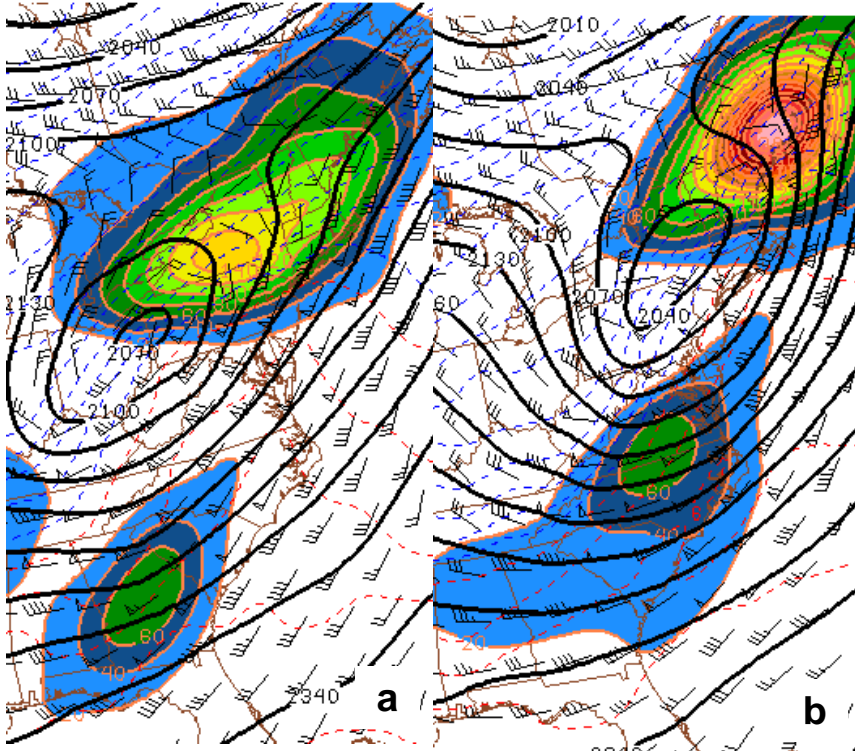
Figure 13: 850-700 hPa mean Pettersson frontogenesis (shaded), mean geopotential height (black contours), mean temperature (red and blue dashed contours), and mean wind barbs for (a) 12 UTC on 25 February, 2011 and (b) 18 UTC on 25 February, 2011.
