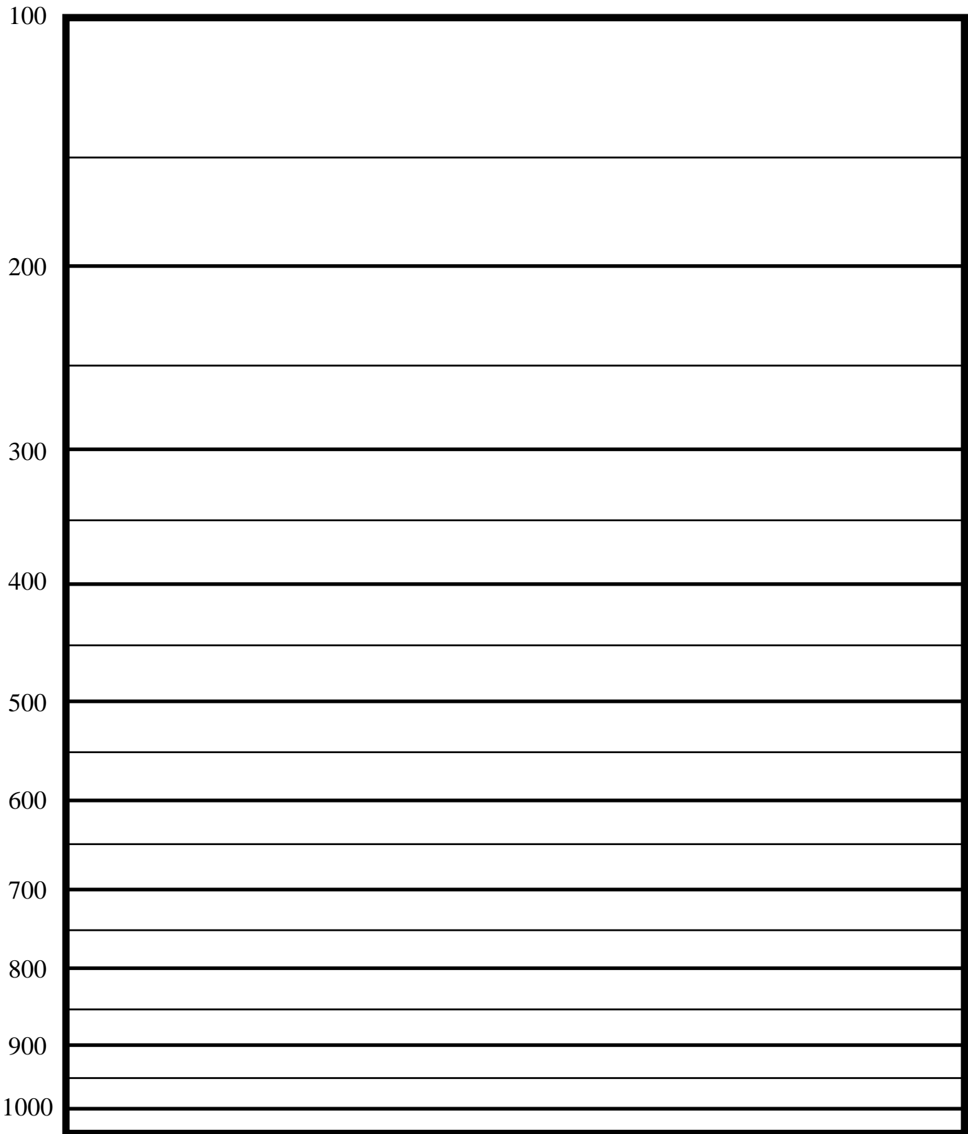
Isobars (Millibars)
