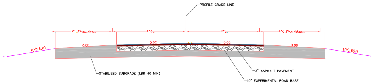
Figure 2-4: Detailed cross section of the demonstration road
