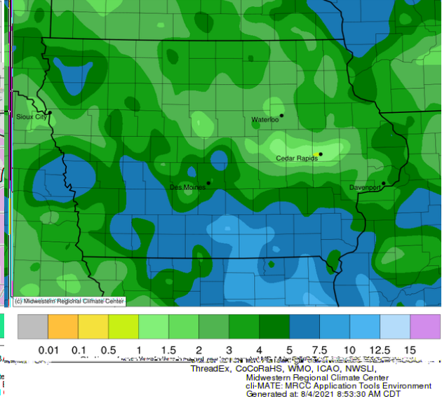
Accumulated Precipitation (in) July 01, 2021 to July 31, 2021
