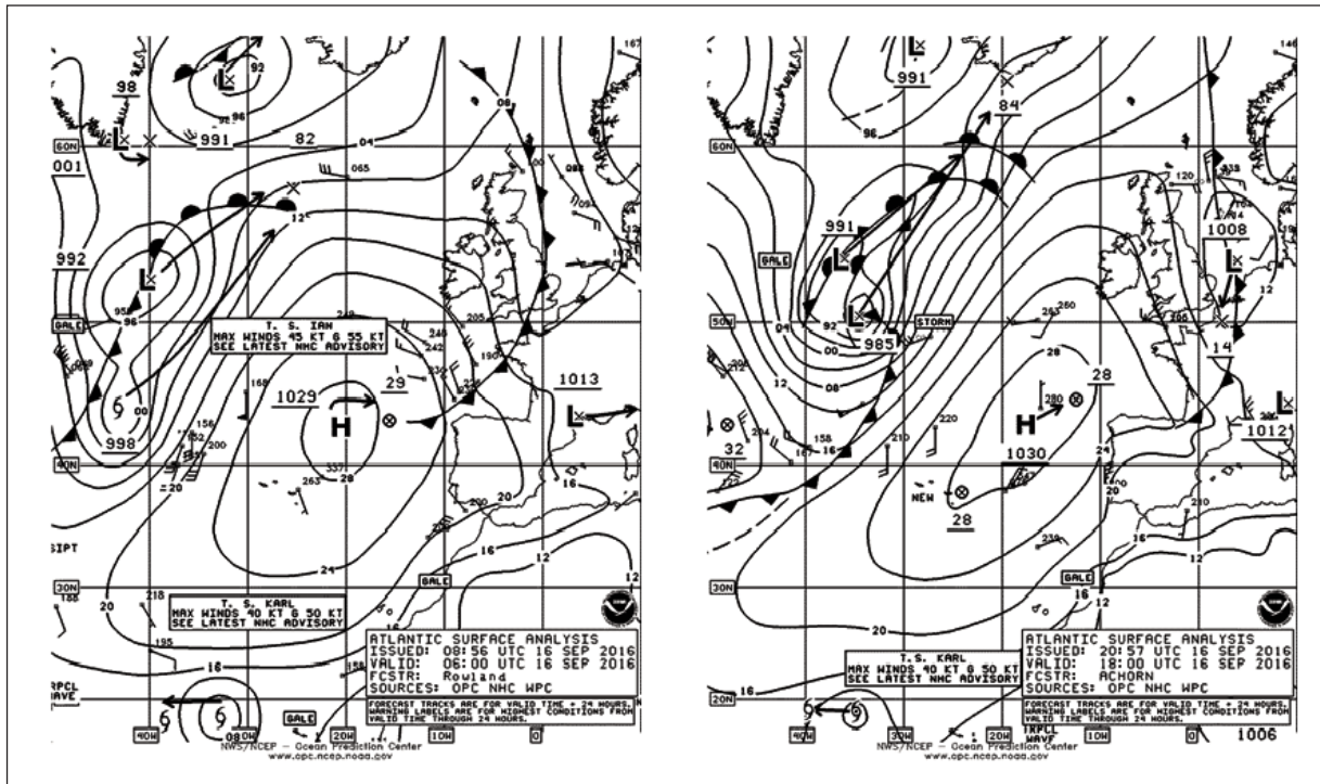
Figure 3. OPC North Atlantic Surface Analysis Charts (Part 1 — East) valid 0600 and 1800 UTC September 16, 2016.
