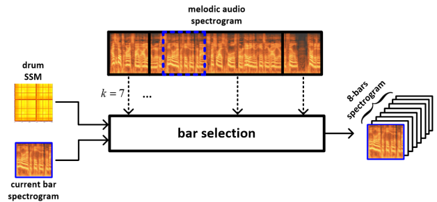
Figure 3. Bar selection mechanism to pick spectrogram data from the current and the other 7 relevant bars.
