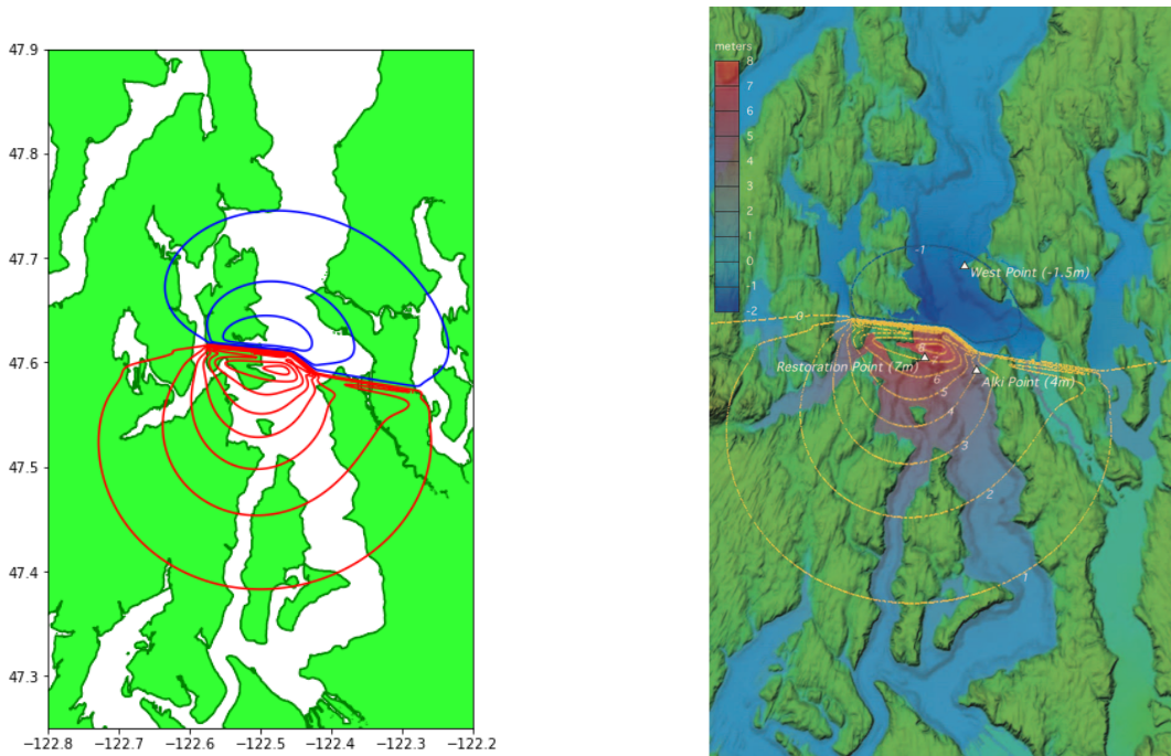
Figure 13: Left: SF-L deformation provided by PMEL and used in Snohomish County study. Right: Figure 2 from PMEL-124 [32]. Note that the contours in the figure on the right match well with those on the left and with those of Figure 14, and not so well with those shown on the left in Figure 15. This suggests a fault width of 35 km might have been used in [32], contrary to the table in that report.
