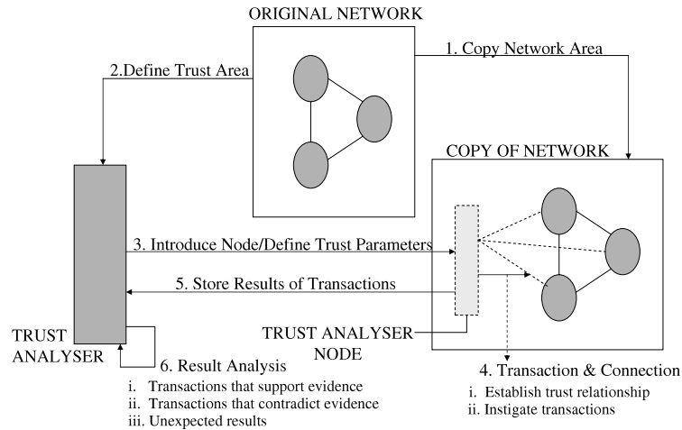
Figure 1. Using trust models to gather forensic evidence.
