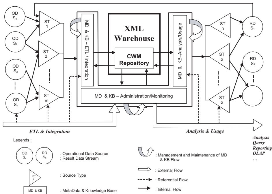
Figure 1: Complex Data Warehouse Architecture Framework
