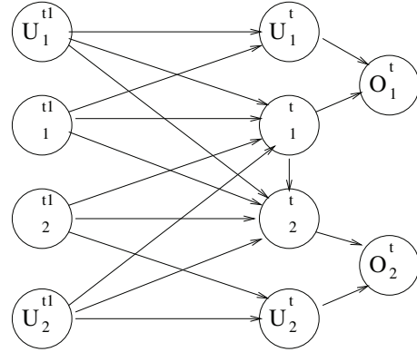
Figure 1: DBN representation of two-entity GLDM.
