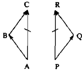
Figure 2 Two independent penguin triangles
