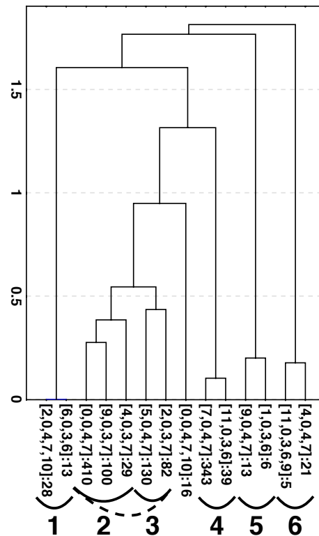
Figure 3. (a) The dendrogram derived from the Euclidean distances between rows of the transition matrix (Figure 2).
