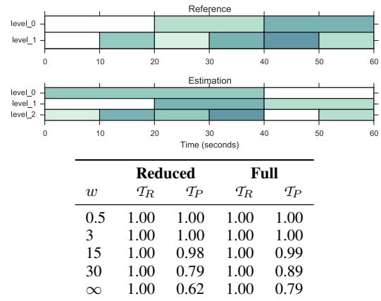
Figure 7: 2-layer vs. 3-layer hierarchical boundaries (top) and T -measures scores (bottom).
