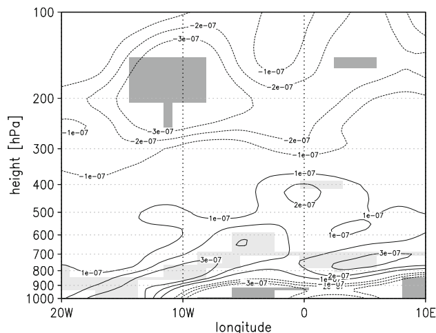
Fig. 14 Cross section of the summer (JAS) horizontal wind divergence anomalies averaged from 12°N to 20°N for the Indian Ocean experiment (1/s). The x-axis shows the longitude and the y-axis the height. The contours indicate the horizontal divergence. Positive values mean divergence and negative convergence. The shading denotes significant changes at the 95% significance level according to a two-tailed t test
