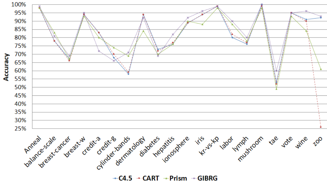
Figure 2: Accuracy comparison
