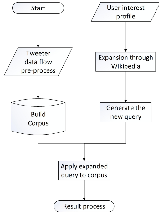
Figure 1: System framework.
