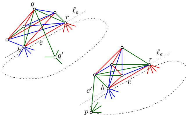
Figure 3: Two examples depicting the construction of three edge-disjoint plane spanning trees on S .
