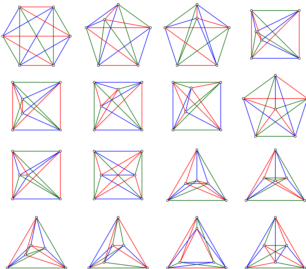
Figure 8: The 16 combinatorially different point sets for n = 6 [3, 2], with 3 edge-disjoint plane spanning trees each.
