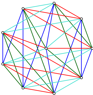
Figure 5: GW_{2n} contains n - 1 plane spanning paths.
