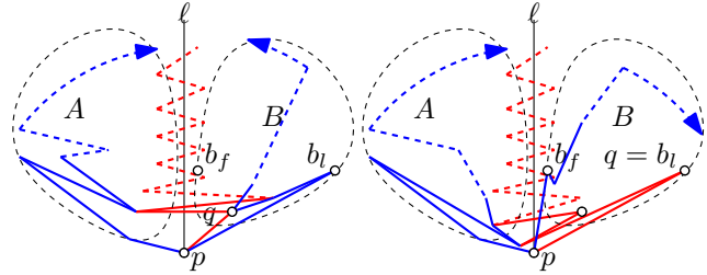
Figure 6: Partition of S \setminus \{p\} and the two edge-disjoint spanning paths. Left: q \neq b_l . Right: q = b_l .
