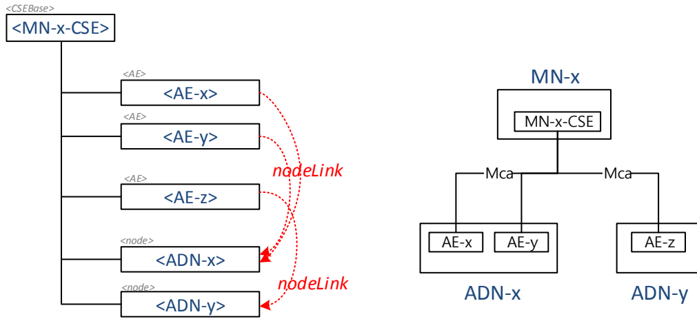
Figure 9.6.18-1: Relationship between MN and ADN
