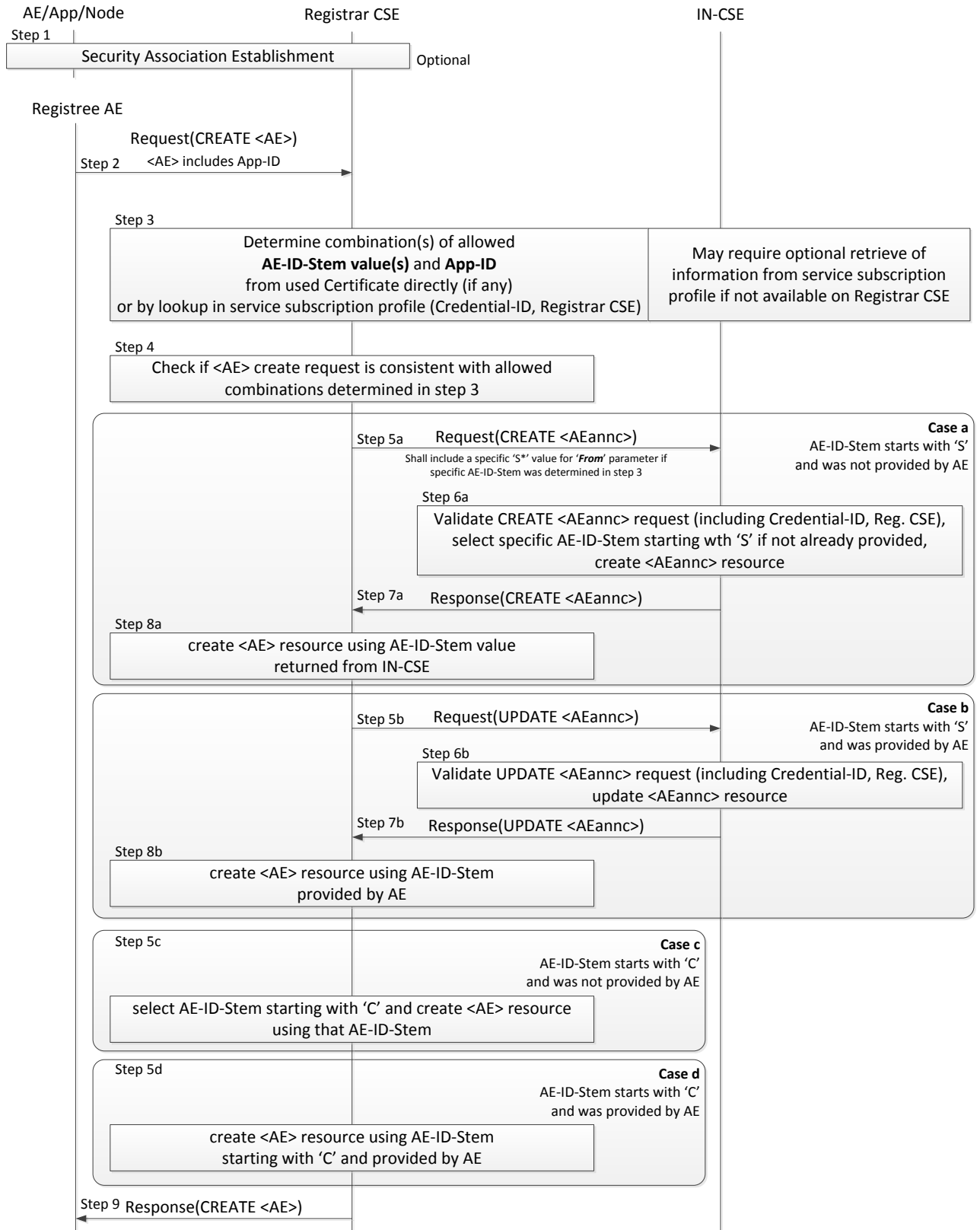
Figure 10.1.1.2.2-1: Procedure for Creating an <AE> Resource
