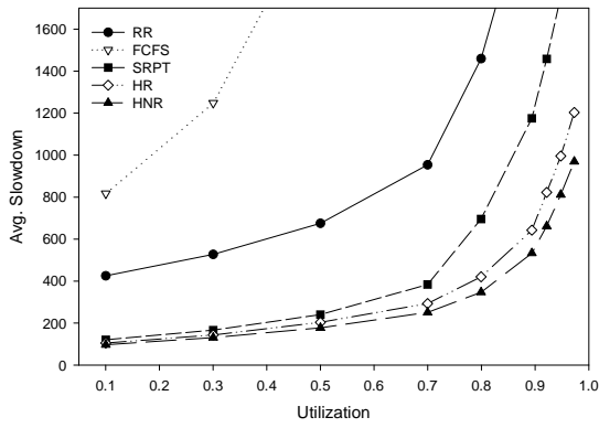
Figure 5: Avg. slowdown vs. system load
