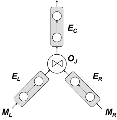
Figure 3: An example of a multi-stream query plan
