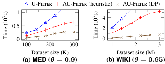
Figure 7: Scalability of proposed join algorithms.
