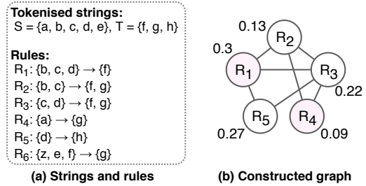
Figure 2: Illustration of Example 5. Numbers beside each vertex is its weight. SQUAREIMP selects R_2 and R_5 , whereas Alg. 1 finally selects R_1 and R_4 .
