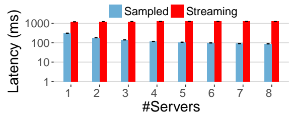
Figure 8: Scalability as we add more servers and increase the dataset proportionally. As before, the ideal scalability corresponds to a constant latency. Note that the Y axis is logarithmic.
