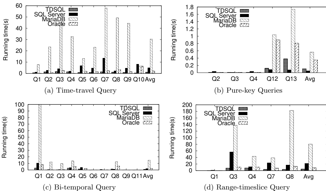
Figure 9: Performance study on TPC-BiH
