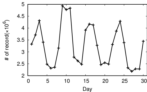
Figure 5: Number of expense statements per day
